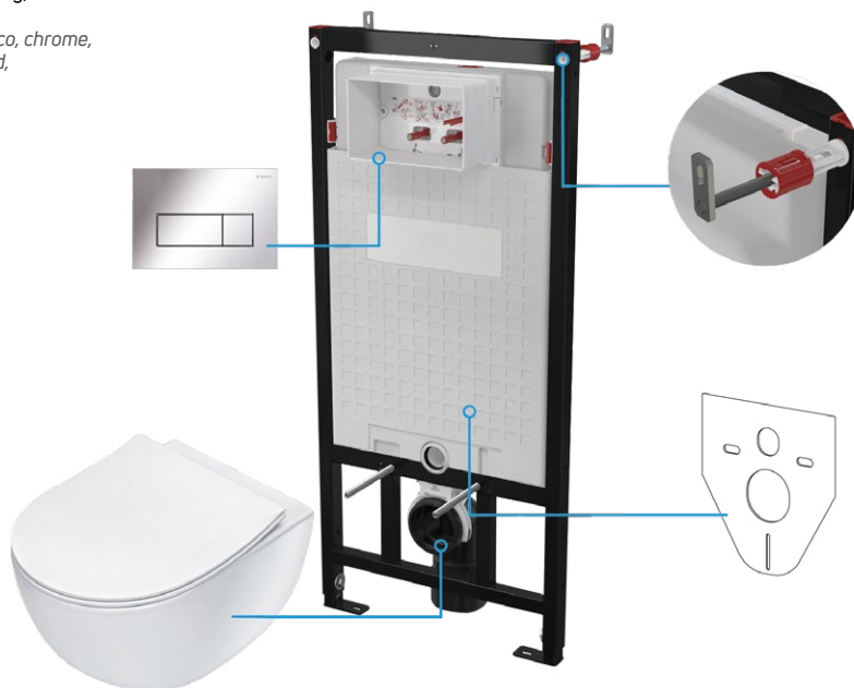
CDET6ZPW TITANIUM, BIAŁY / TITANIUM, WHITE
